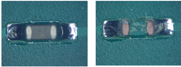
Flux around surface mount Flux under cap
