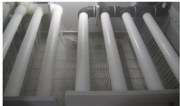
Figure 3: Picture of wash section equipped with progressive energy dynamics
